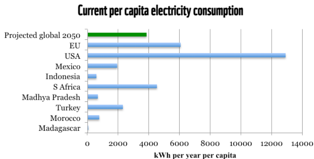
FIGURE 4: 2050 GLOBAL AND CURRENT REGIONAL PER CAPITA ELECTRICITY CONSUMPTION.
