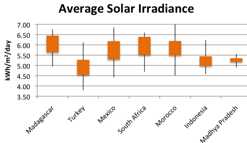
FIGURE 6: EACH OF THE SELECTED REGIONS HAS A “VERY GOOD” TO “EXCELLENT” SOLAR RESOURCE.
