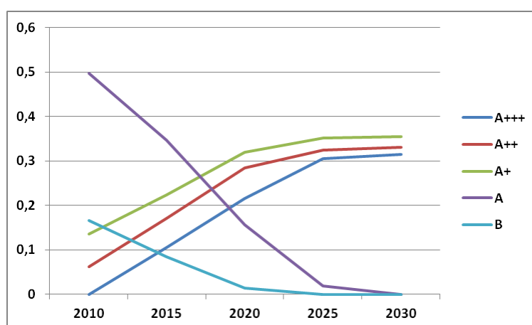
Figure 32: Transformation of the market share of washing machines by energy class in the Base_inclEA Scenario
