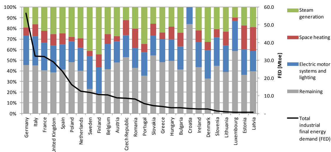
Figure 41: Final energy demand by technology and country in 2010 as share of total industrial final energy demand
