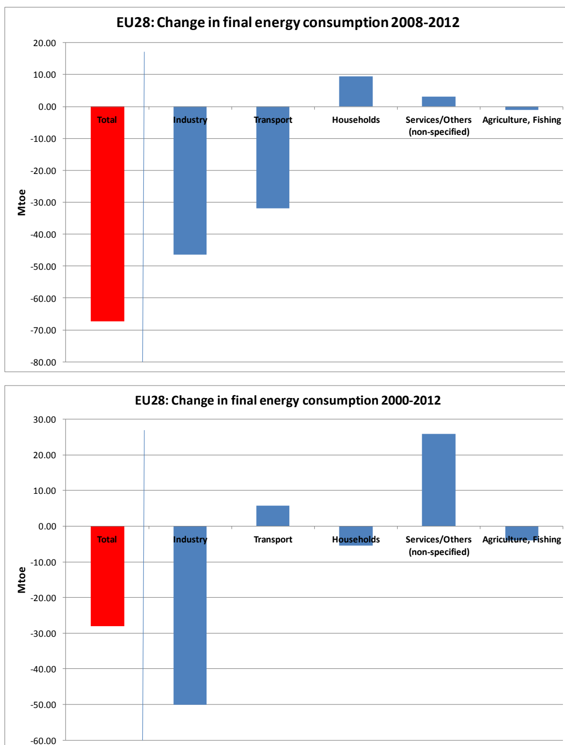
Figure 16: Sectoral decomposition of changes in final energy consumption 2008-2012 and 2000-2012
