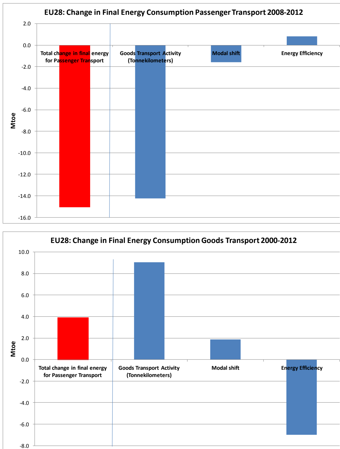
Figure 20: Sectoral decomposition analysis ( goods transport sector ) of changes in final energy consumption 2008-2012 (upper figures) and 2000-2012 (lower figure)
