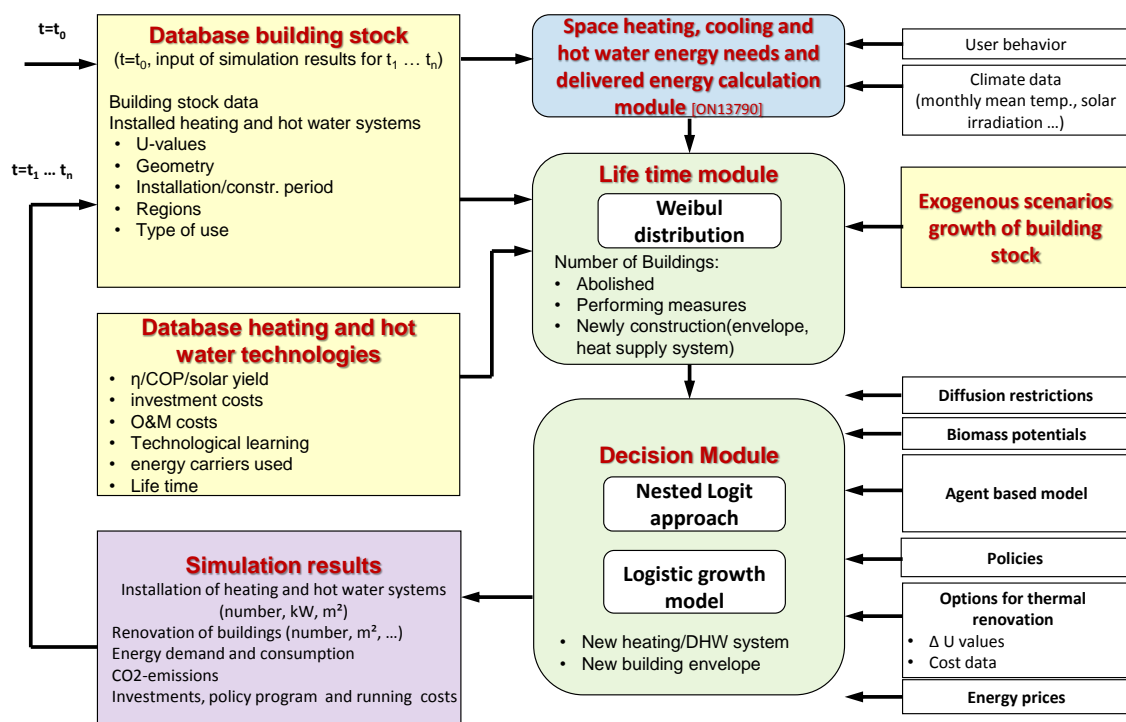
Figure 53: Overview structure of Simulation-Tool Invert/EE-Lab
