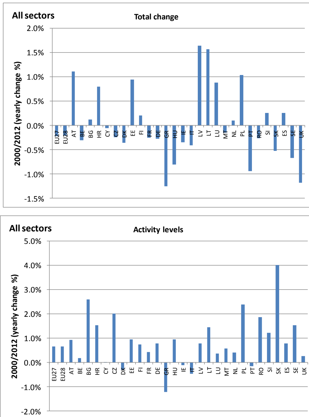
Figure 22: Total change in final energy consumption and different factors 2000-2012 (annual change in percent)
