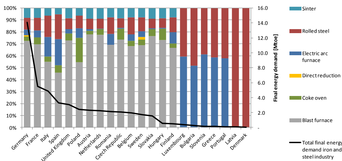
Figure 39: Final energy demand in the iron and steel industry by process and country in 2010
