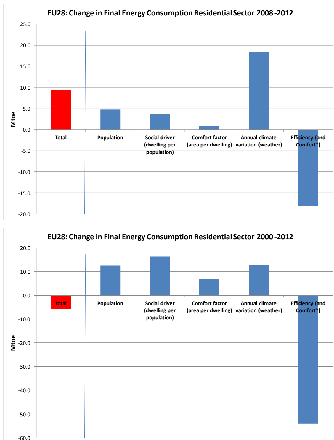
Figure 17: Sectoral decomposition analysis ( residential sector ) of changes in final energy consumption 2008-2012 and 2000-2012 (lower figure)
