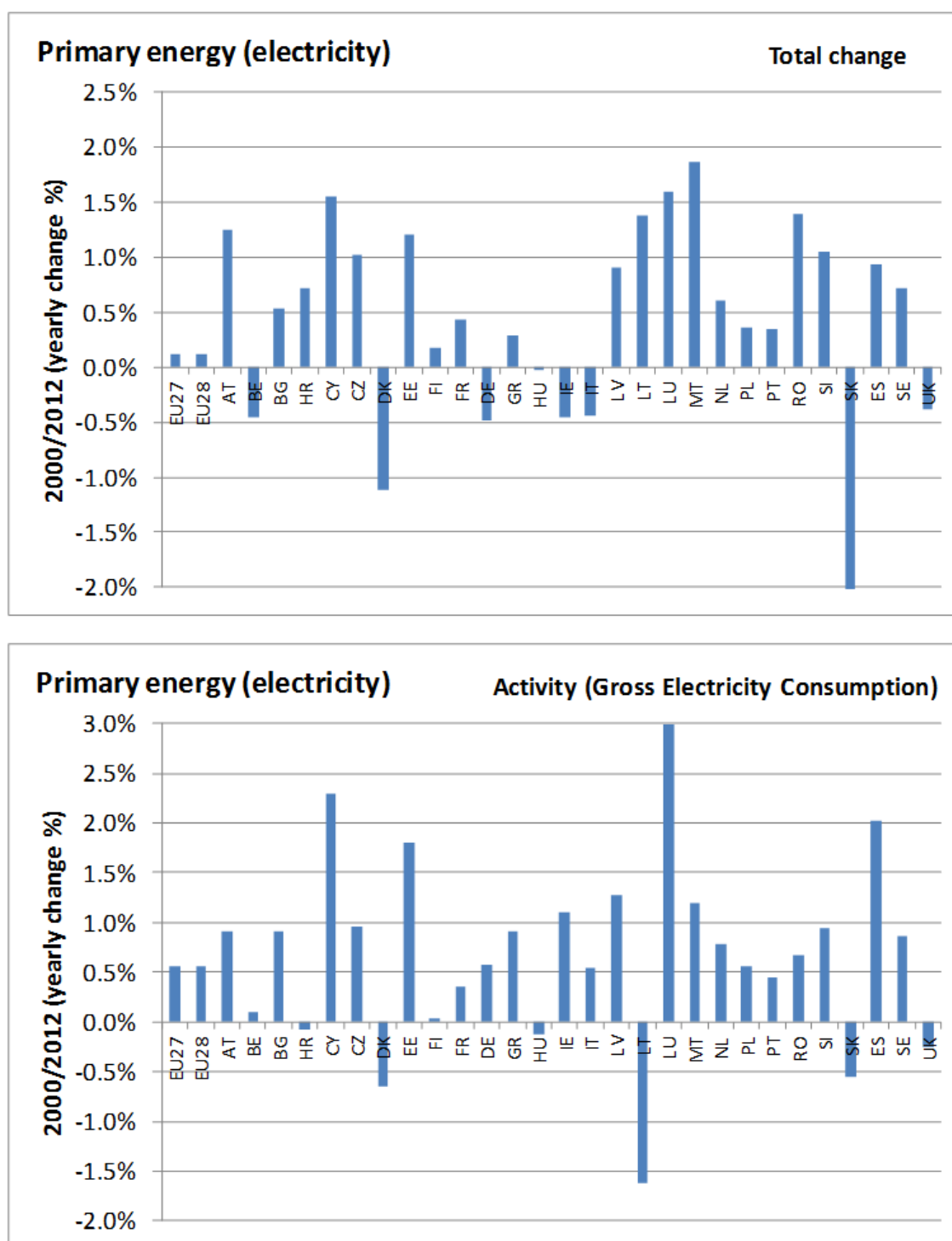
Figure 26: Total change in primary energy consumption for electricity generation and different factors 2000-2012 (annual change in percent)
