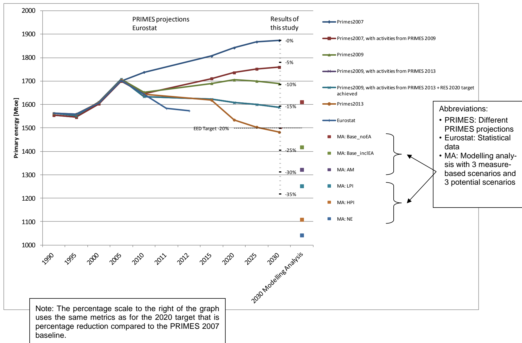
Figure 3: Summary of main results for the primary energy potentials for the EU in 2030
