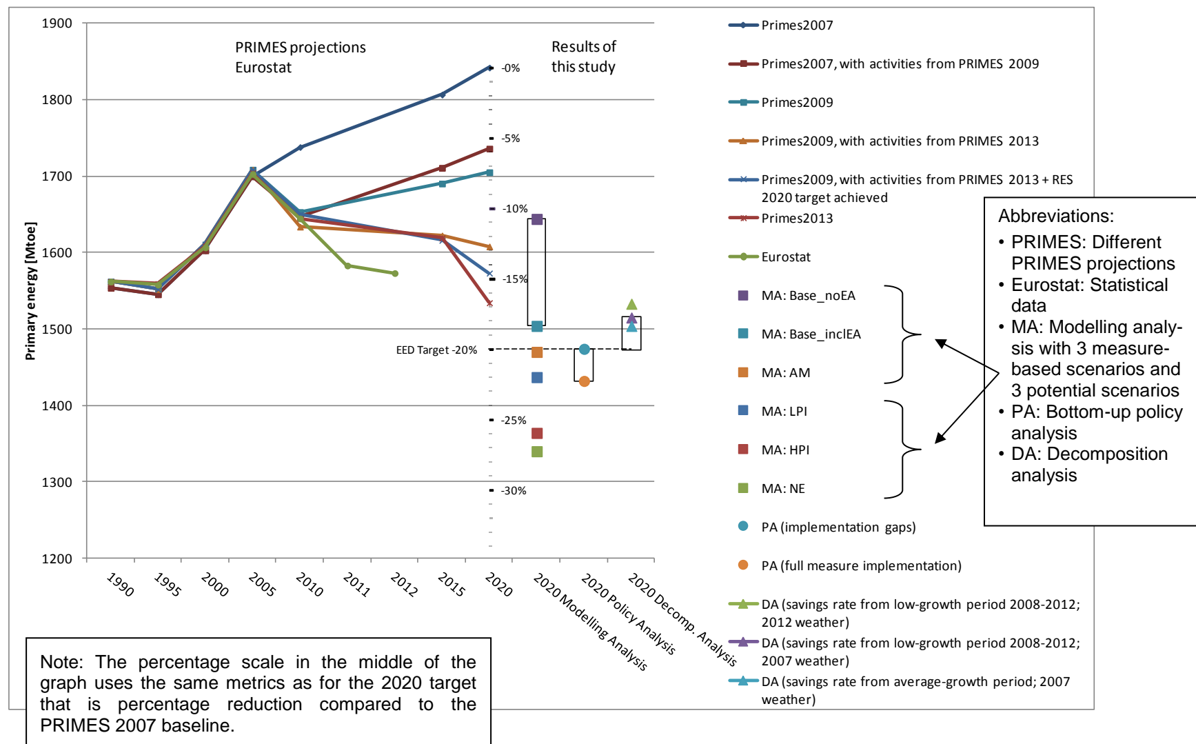
Figure 1: Summary of main results for the projected primary energy gap for the EU in 2020
