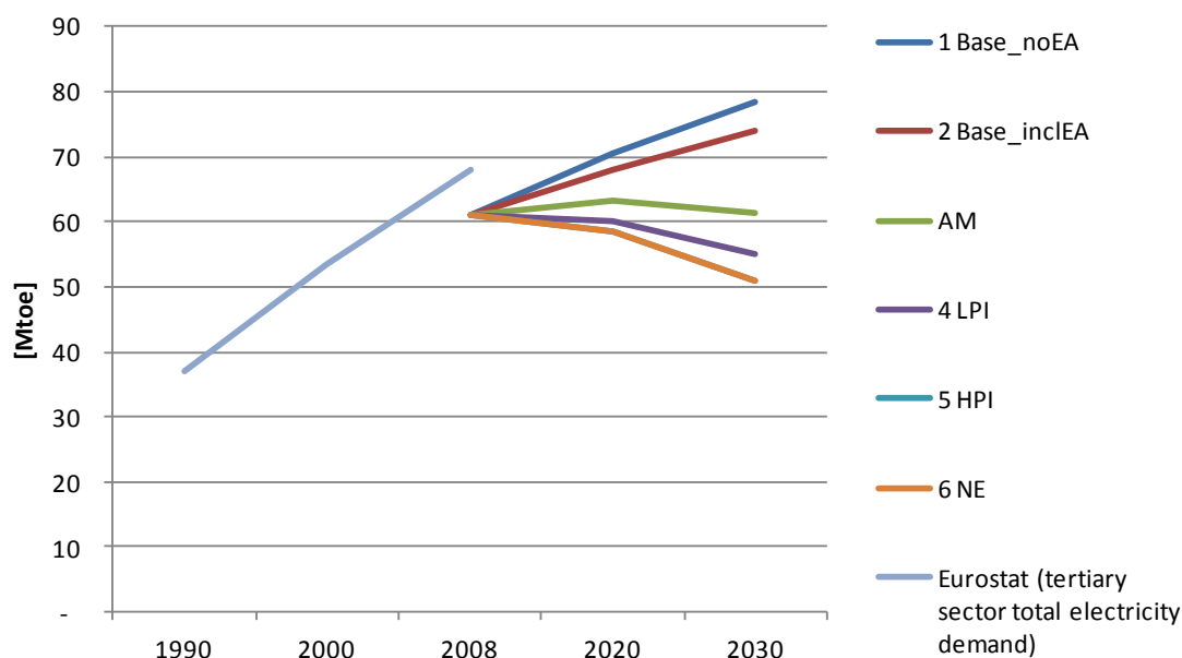
Figure 37: Electricity demand for tertiary sector appliances in EU27 by scenario (the gap between historic electricity demand and projections is explained by space heating and hot water demand – see section 5.5.1)
