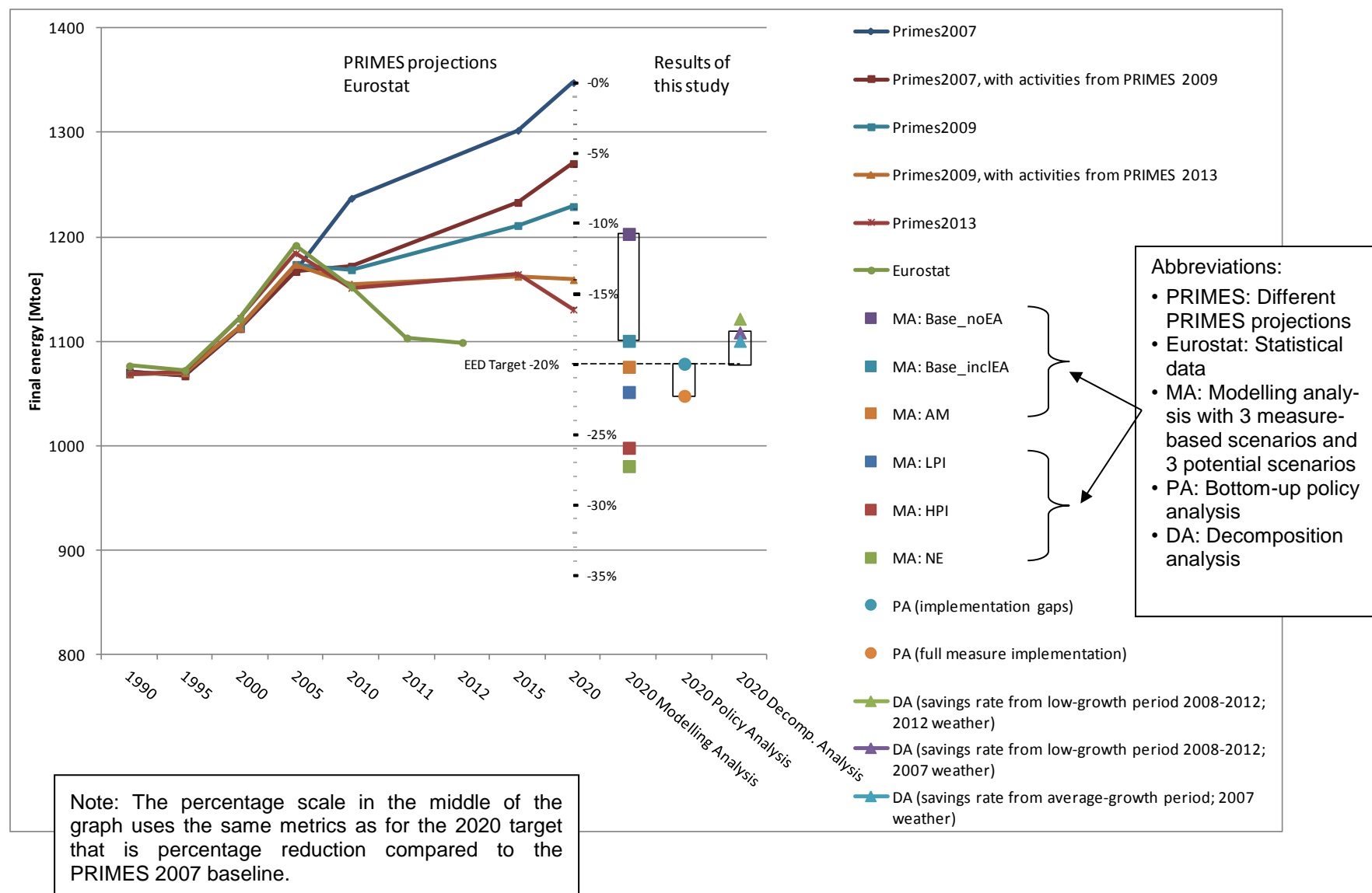
Figure 2: Summary of main results for the projected final energy gap for the EU in 2020
