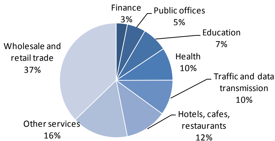
Figure 33: Sub-sectors considered in FORECAST-Tertiary and their share of EU28 electricity demand in 2008
