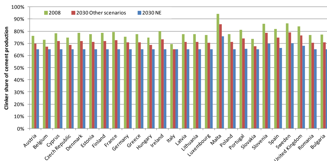
Figure 46: Clinker share in 2008 and by scenario in comparison
