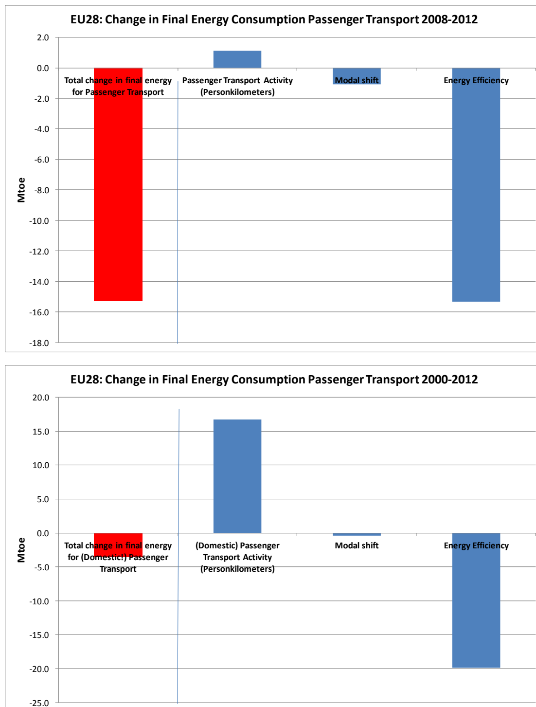
Figure 19: Sectoral decomposition analysis ( passenger transport sector ) of changes in final energy consumption 2008-2012 (upper figures) and 2000-2012 (lower figure)
