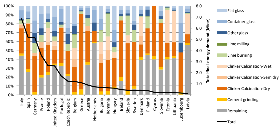
Figure 40: Final energy demand in the non-metallic mineral industry by process and country in 2010
