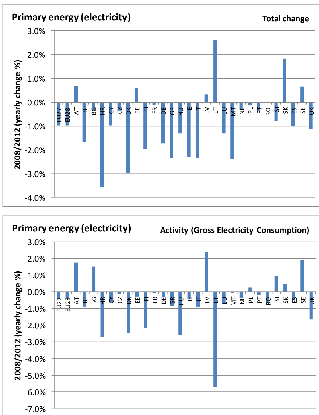
Figure 27: Total change in primary energy consumption for electricity generation and different factors 2000-2012 (annual change in percent)
