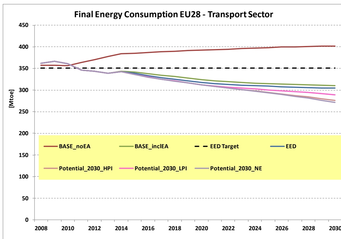
Figure 38: Overview on final energy consumption of the transport sector in each scenario for EU28
