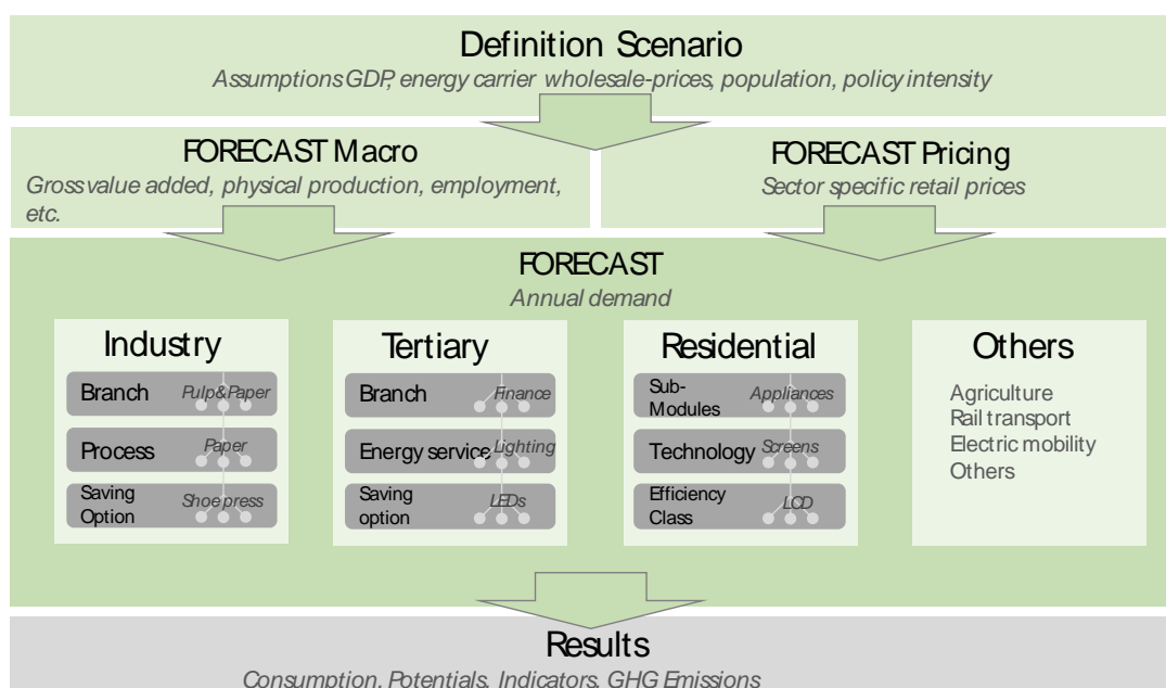
Figure 52: Overview of FORECAST model structure
