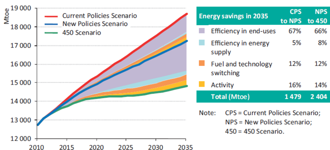
Figure 49: Energy efficiency contributions from the supply and the demand side at the world level
