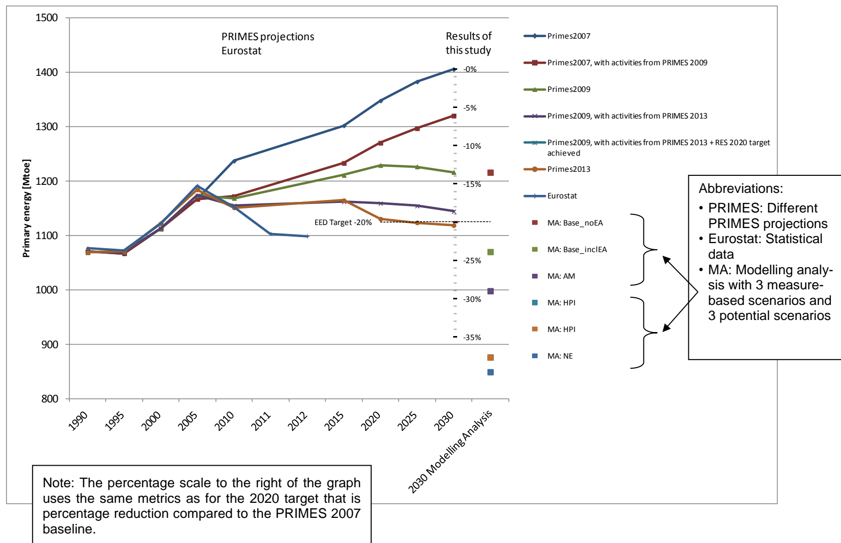
Figure 4: Summary of main results for the final energy potentials for the EU in 2030
