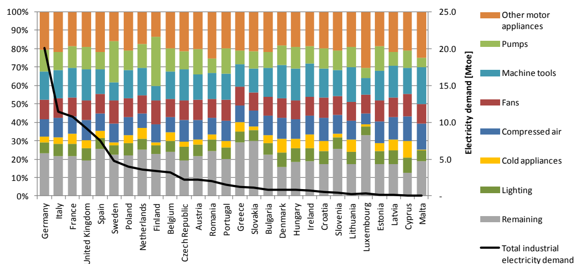
Figure 42: Electricity demand by cross-cutting technology (CCT) and country in 2010 as share of total industrial electricity demand
