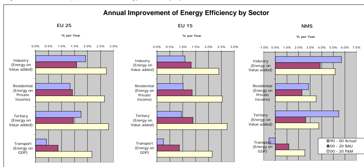
Figure 2: Annual Improvement of Energy Efficiency by Sector
