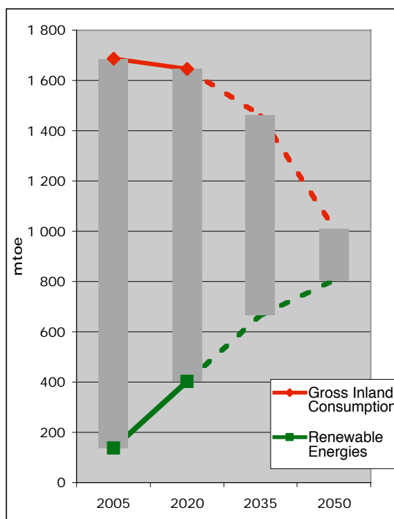
Figure 5: Gross Inland Energy Consumption and Renewable Energy Sources – Long Term Strategy for the EU 25 Until 2050
