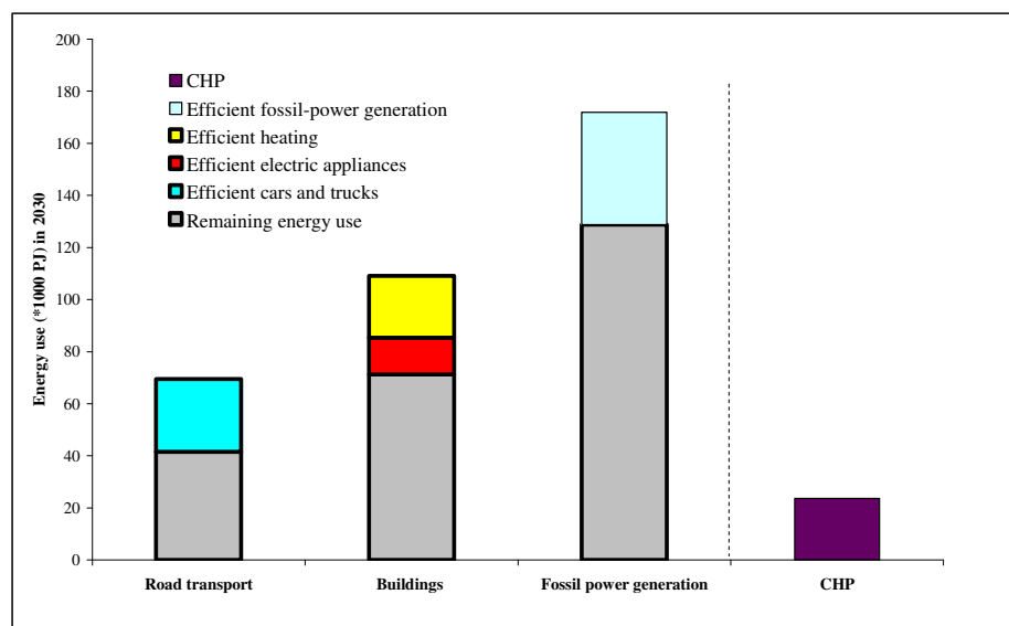
Figure 1 Potential for energy-efficiency improvement in 2030 for the G8 plus 5 countries compared to the Reference Scenario.
