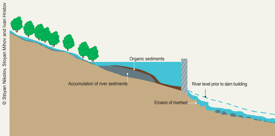
Fig. 19. Changes in sediment transport resulting from dams
