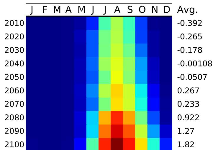
Sea surface temperature
