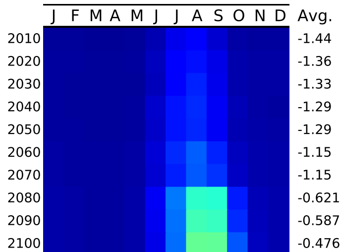
Sea surface temperature
