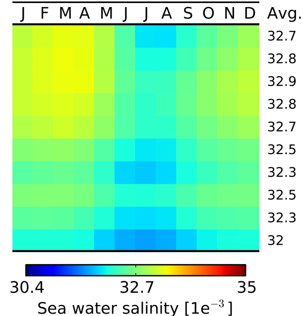
Sea water salinity
