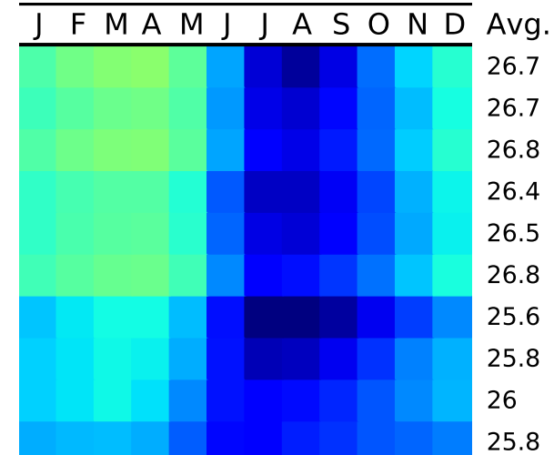
Sea water salinity
