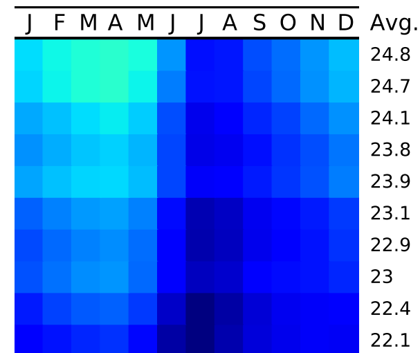
Sea water salinity
