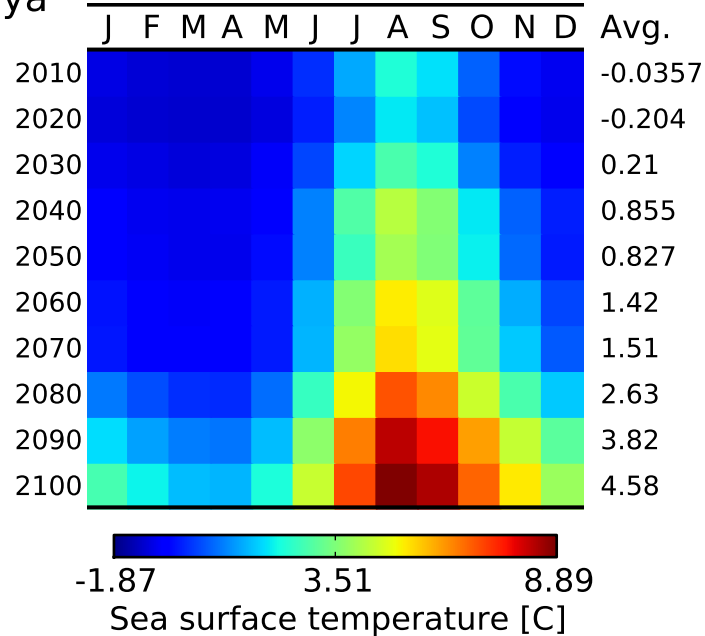
Sea surface temperature
