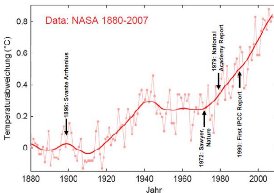
Figure 1 Increase in global mean surface temperature: ~0,8°C (Source: S. Rahmstorf 2008: The 5 most important data sets of climate science) i
